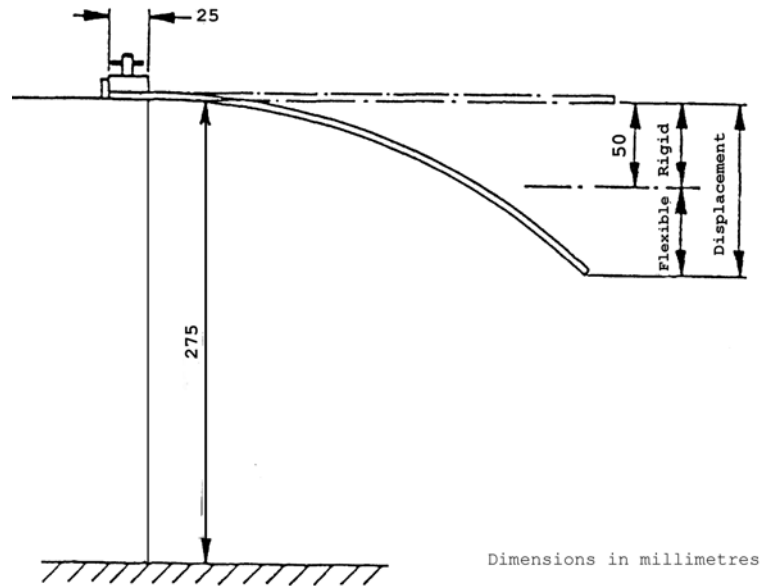
Figure 23: Arrangement of flexibility test
