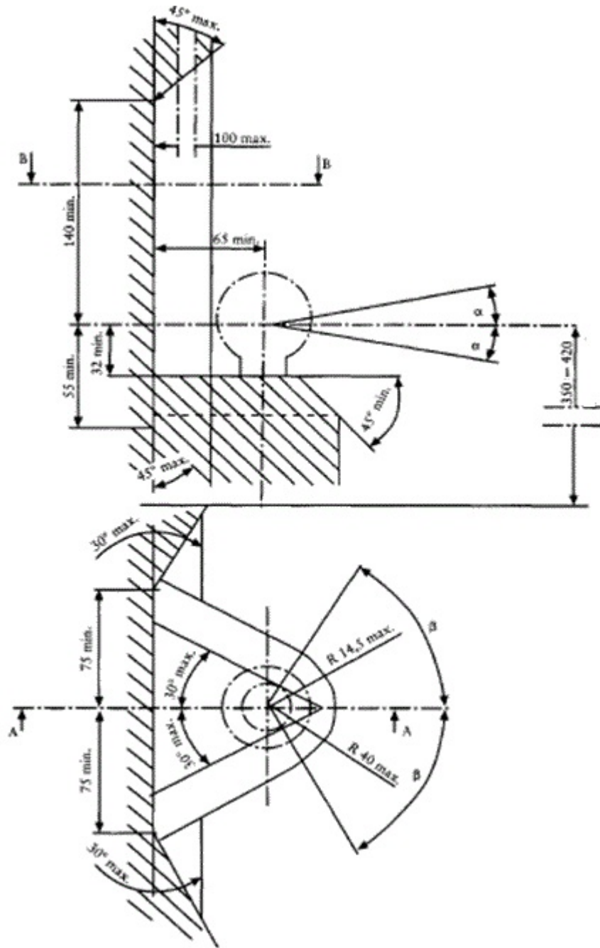
Figure Ap1-2: Clearing space for coupling balls
