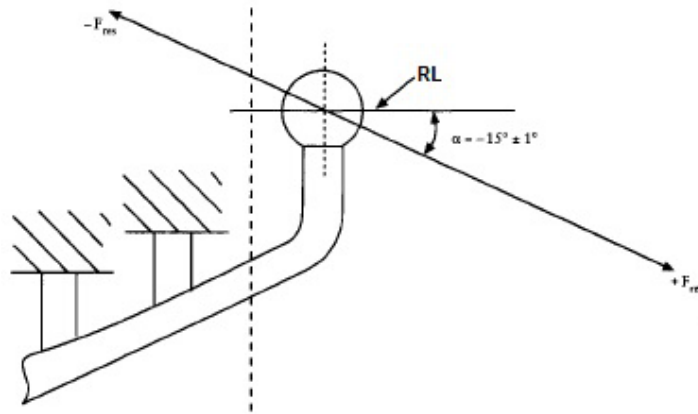
Figure Ap2-1: Dynamic test direction on coupling ball and towing bracket—Test rig I. RL = reference line.
