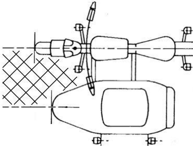
Figure 8-1: Top-down view of category L4e motorcycle with side-car
