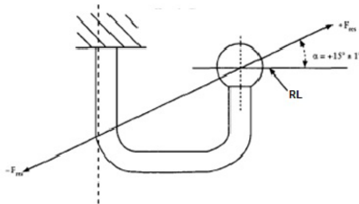
Figure Ap2-2: Dynamic test direction on coupling ball and towing bracket—Test rig II. RL = reference line.
